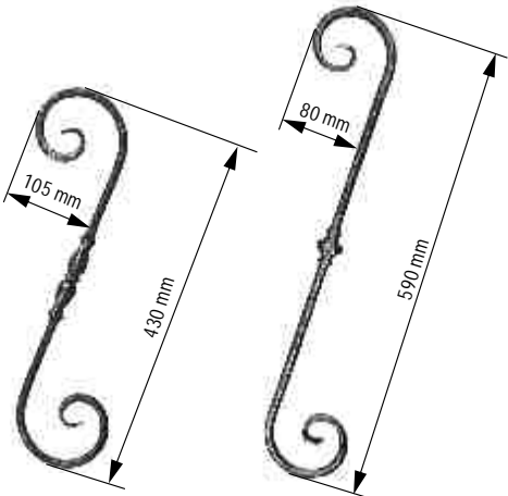
091.33.523 ● 14 mm ↓ 450 mm | € 3.22 ↔ 110 mm | € 2.58 +50 Pz. ⚖️ 1.16 kg
